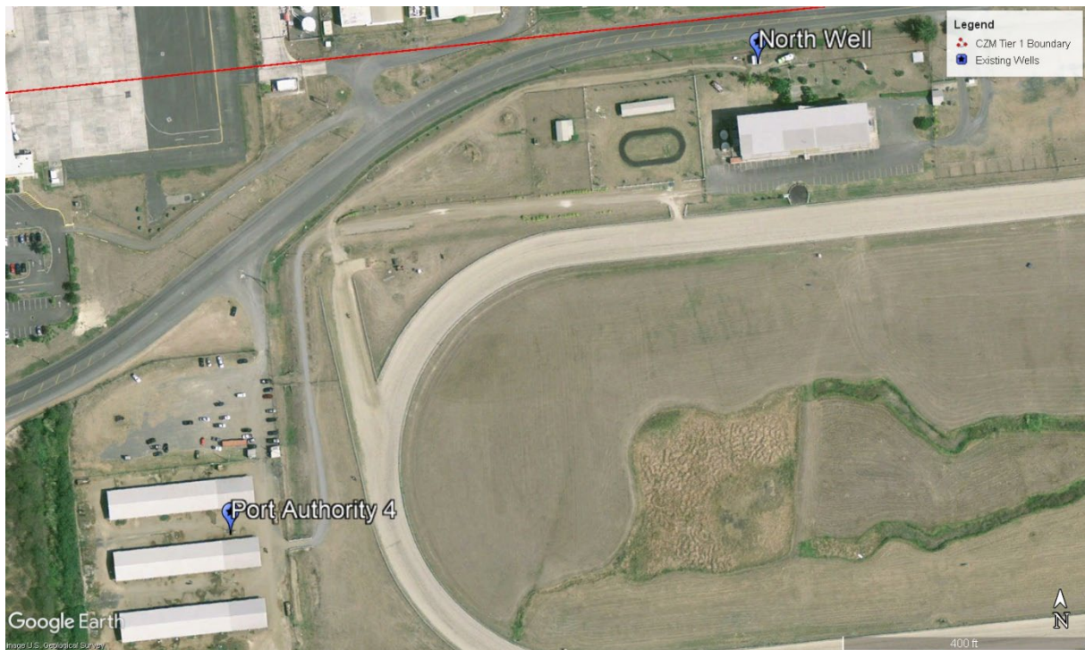
Figure 6.03.2 – Wetland Inventory. U.V.I. - Eastern Caribbean Center/Conservation Data Center, 2000.
