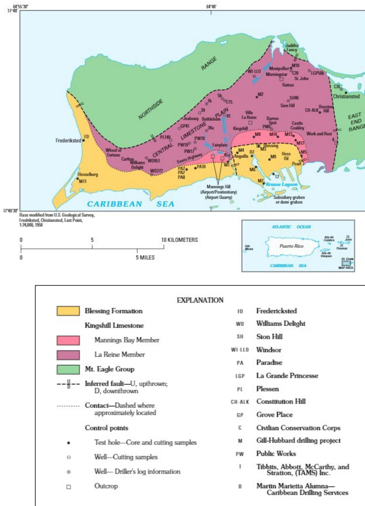
Figure 6.02.3 –Generalized Geology of St. Croix, U.S. Virgin Islands, and location of control points – Renken, 1989
