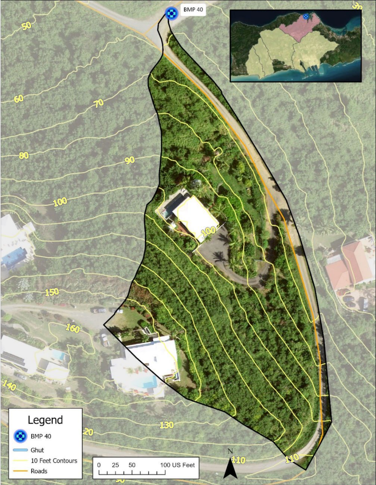
Figure 71. Map depicting the drainage area for BMP 40.
