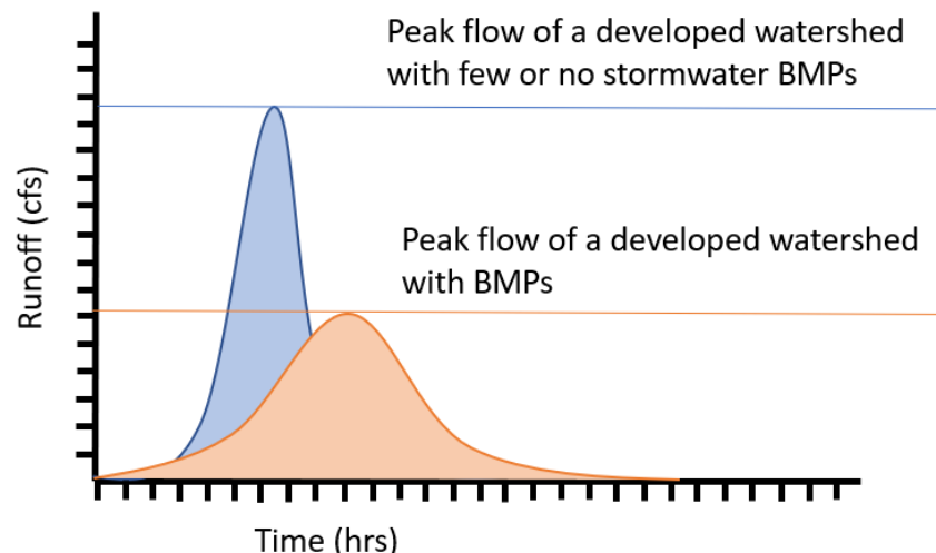
Figure 74. Illustrative hydrographs demonstrating the peak flow reduction value of implementing BMPs.
