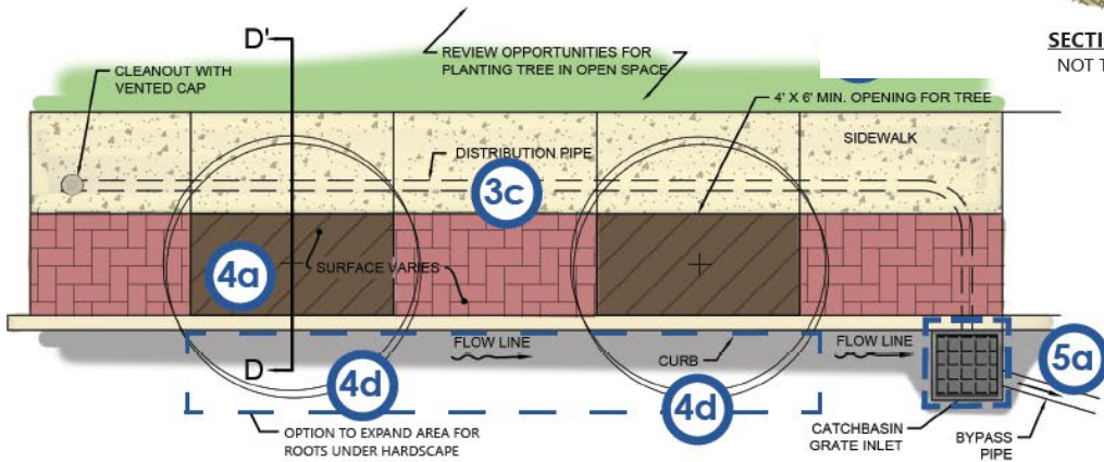
TREE WELL NOT TO SCALE
