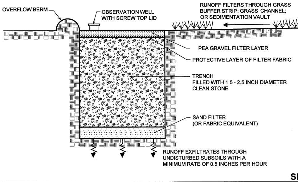
Figure 5.5 Example Infiltration Trench (from RIDEM and CRMC, 2015 – Adapted from MDE, 2000)
