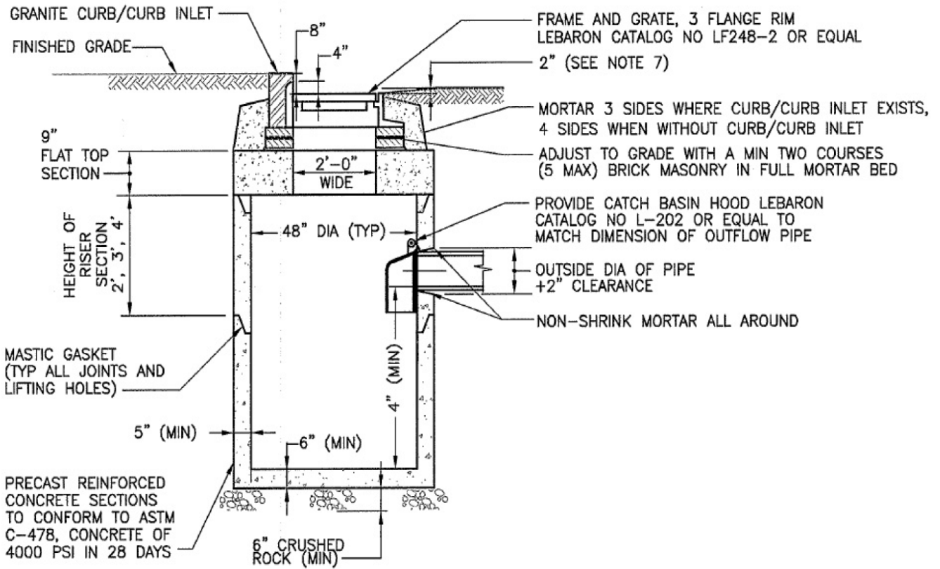
Figure 5.20 Deep Sump Catch Basin (MADEP, 2008)
