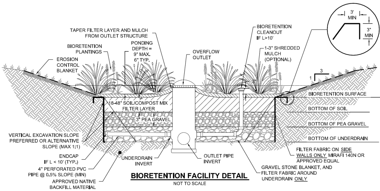
BIORETENTION FACILITY DETAIL NOT TO SCALE
