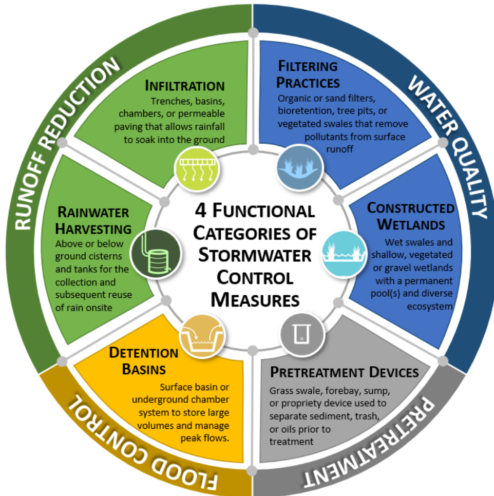
Figure 5.1 The four functional categories of Post-construction Stormwater Control Measures (SCMs).
