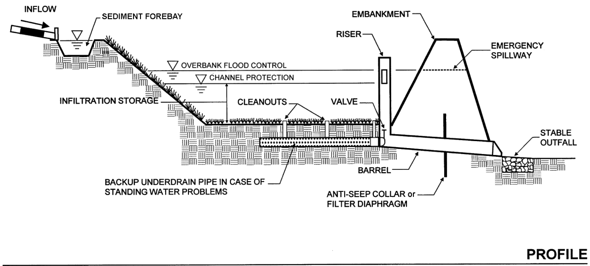
Figure 5.4 Example Infiltration Basin (from RIDEM and CRMC, 2015 – Adapted from MDE, 2000)
