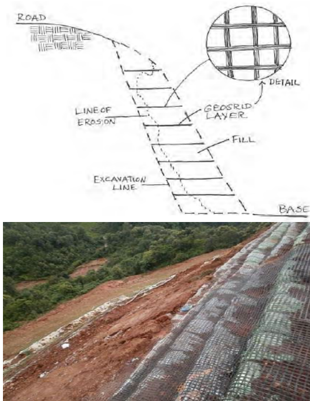
Figure 4.15 Geogrids layers stacked with fill to stabilize a slope (detail from VT Better Backroads Manual).
