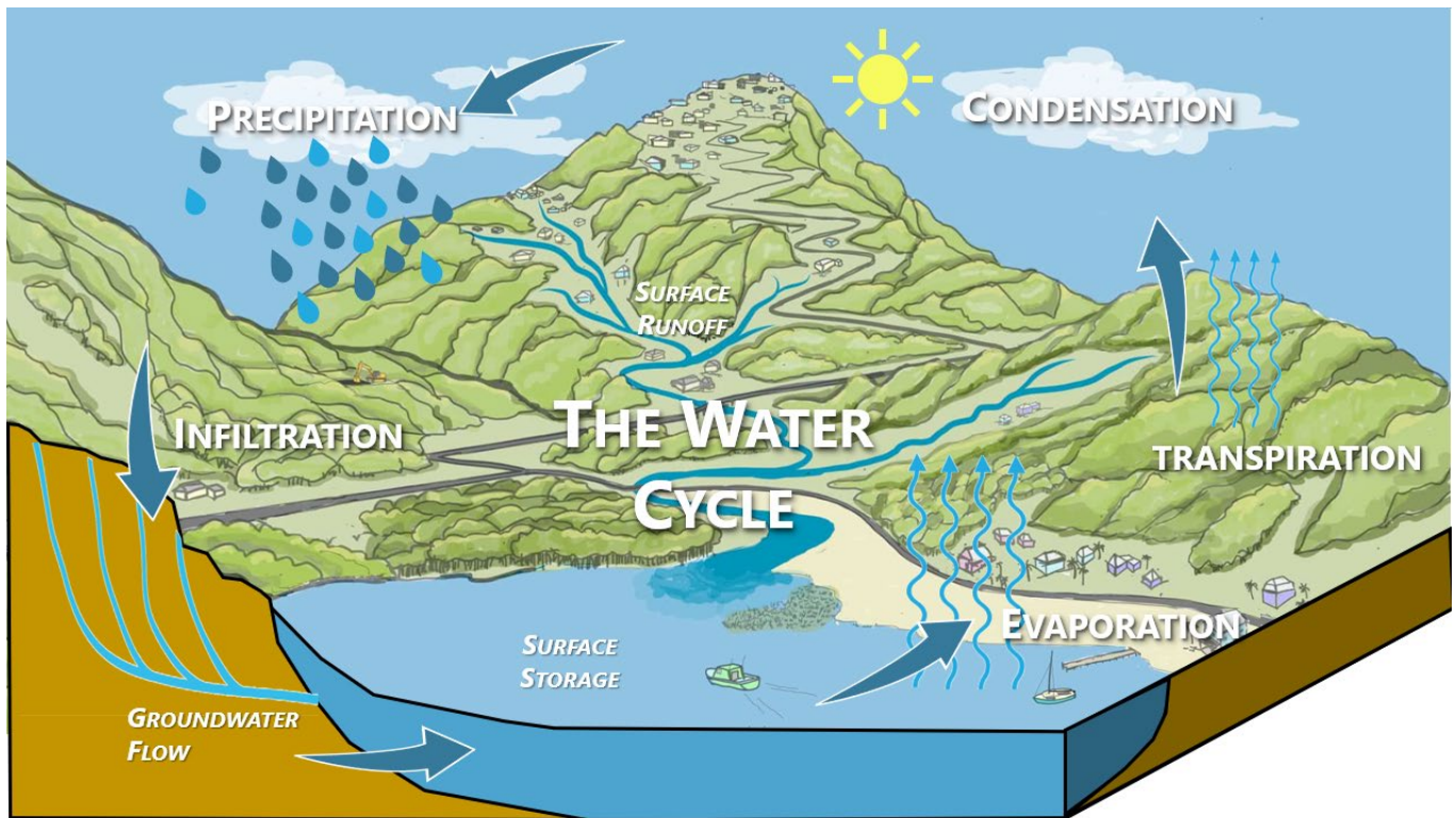
Figure 1.1 The hydrologic cycle (adaptation of graphic created by the Coral Bay Community Council)
