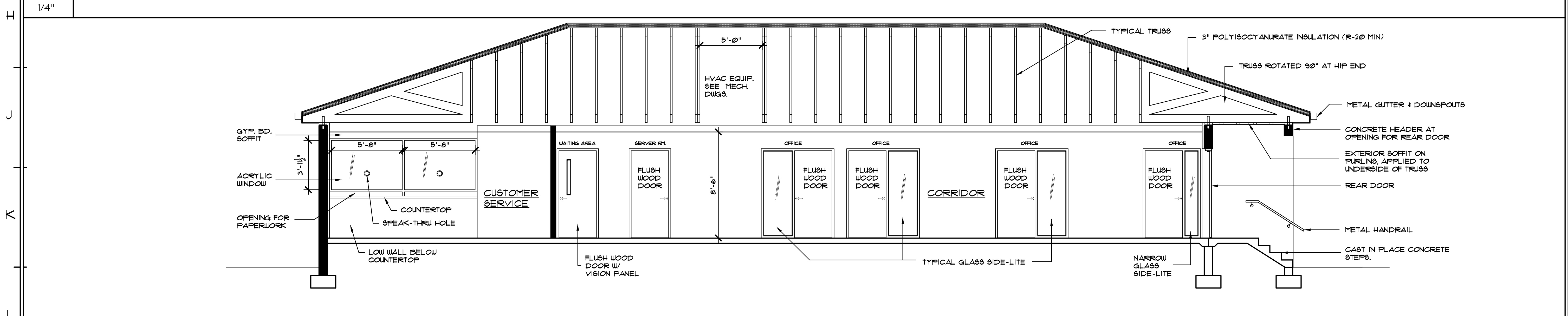
L1 SECTION / INTERIOR ELEVATION AT CORRIDOR (FACING NORTH)
