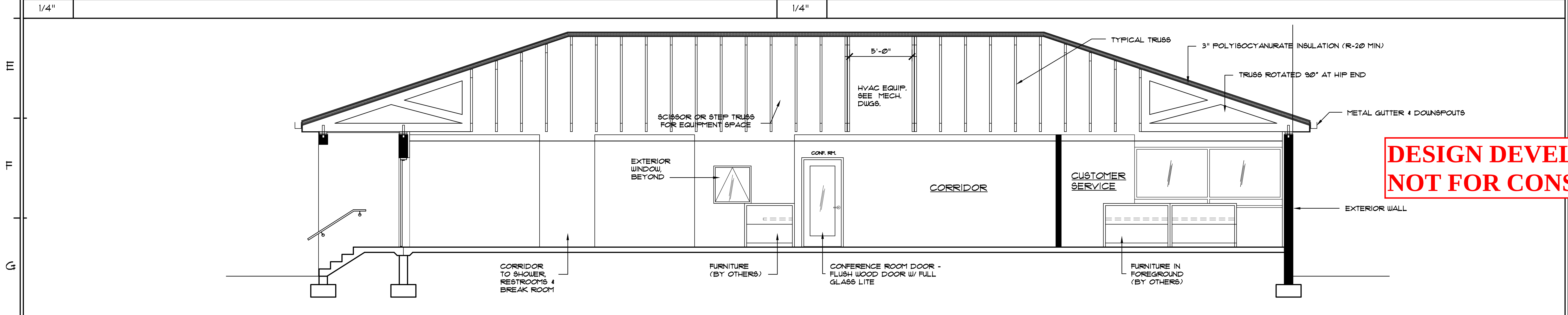
H1 SECTION / INTERIOR ELEVATION AT CORRIDOR (FACING SOUTH)
