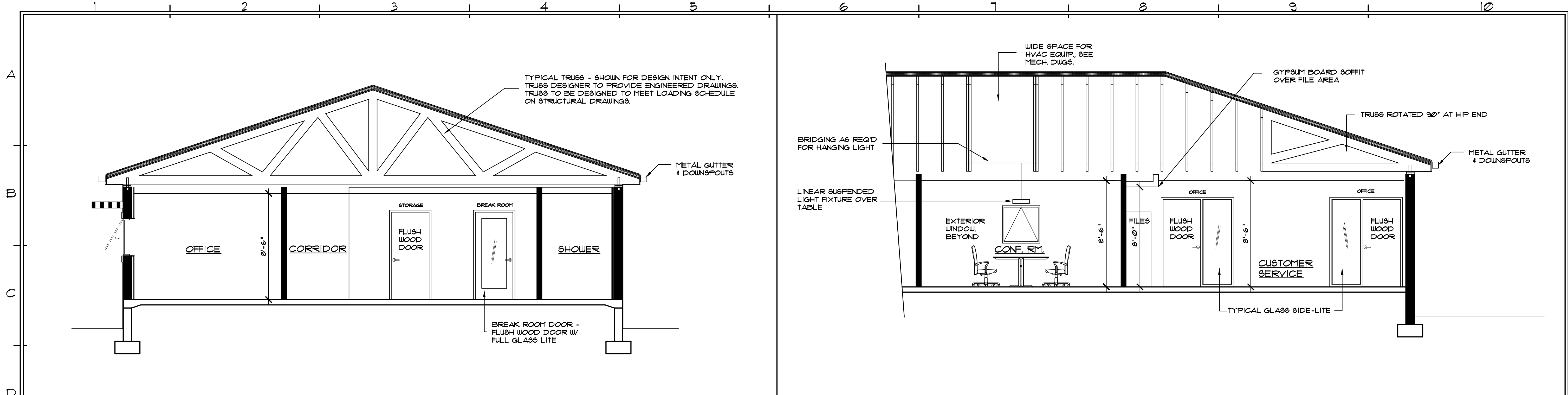
D1 SECTION / INTERIOR ELEVATION AT CONF. ROOM & CUST. SVC.
