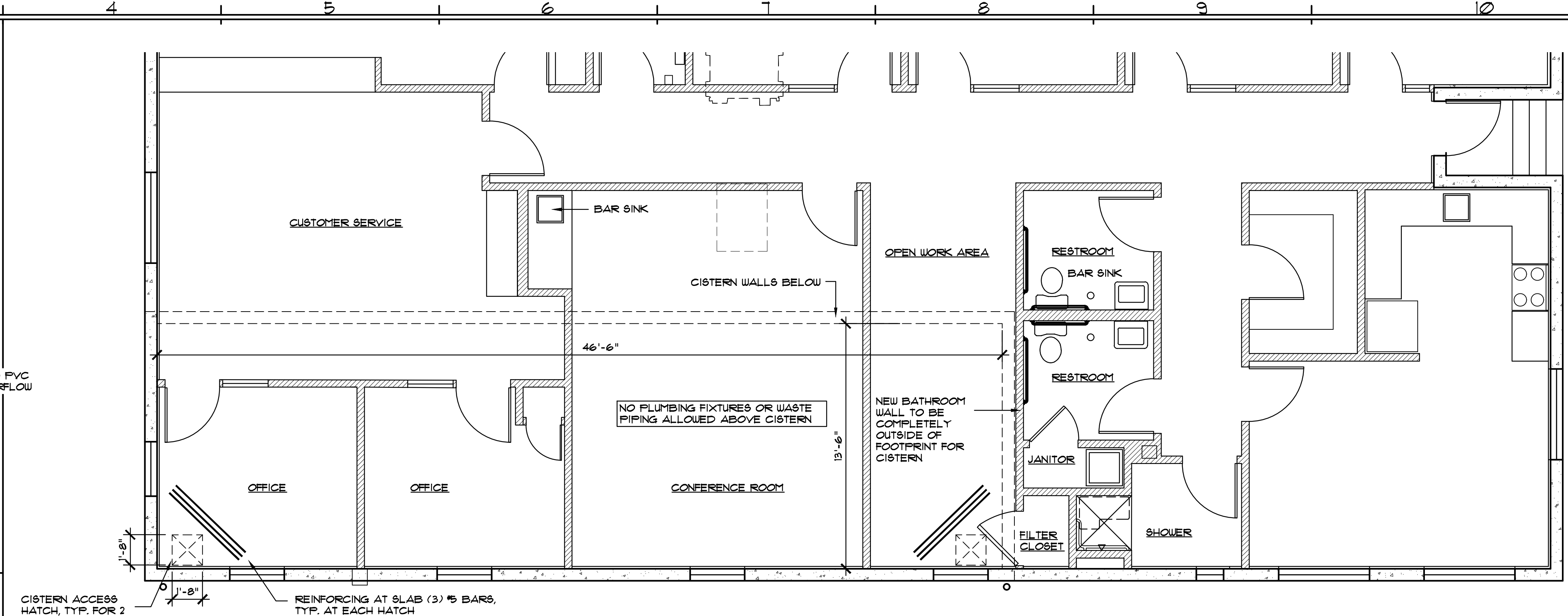
E4 PARTIAL FIRST FLOOR PLAN
