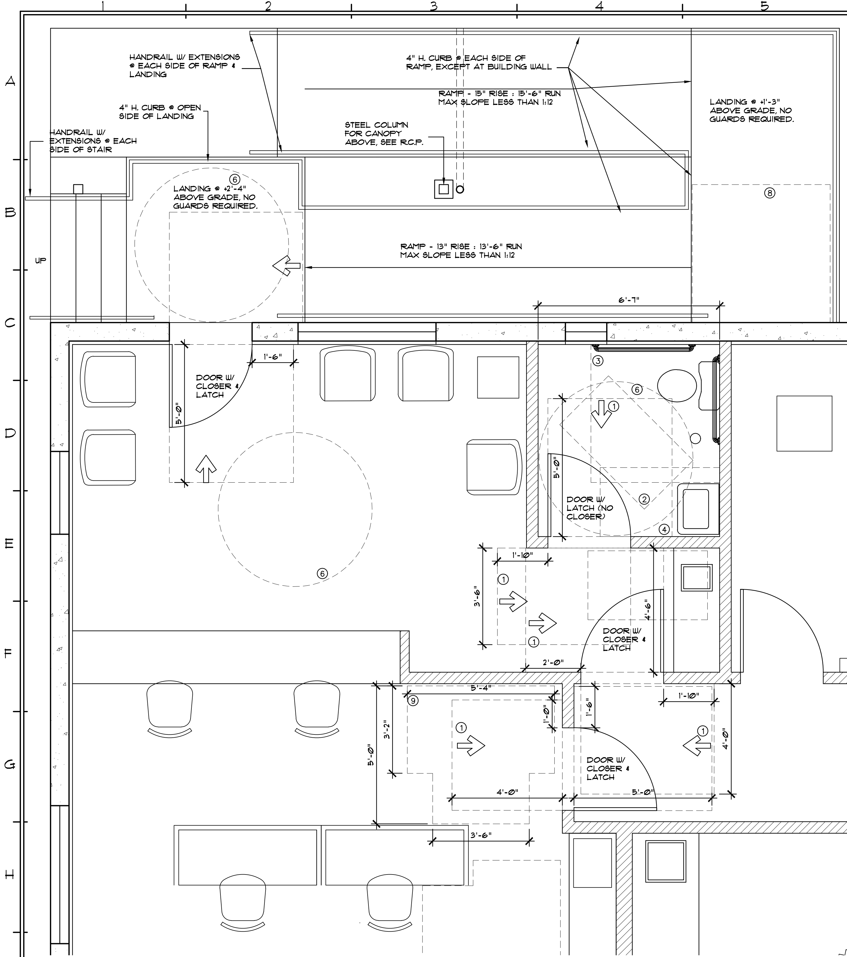
J1 ADA CLEARANCES - LOBBY & CUSTOMER RESTROOM
