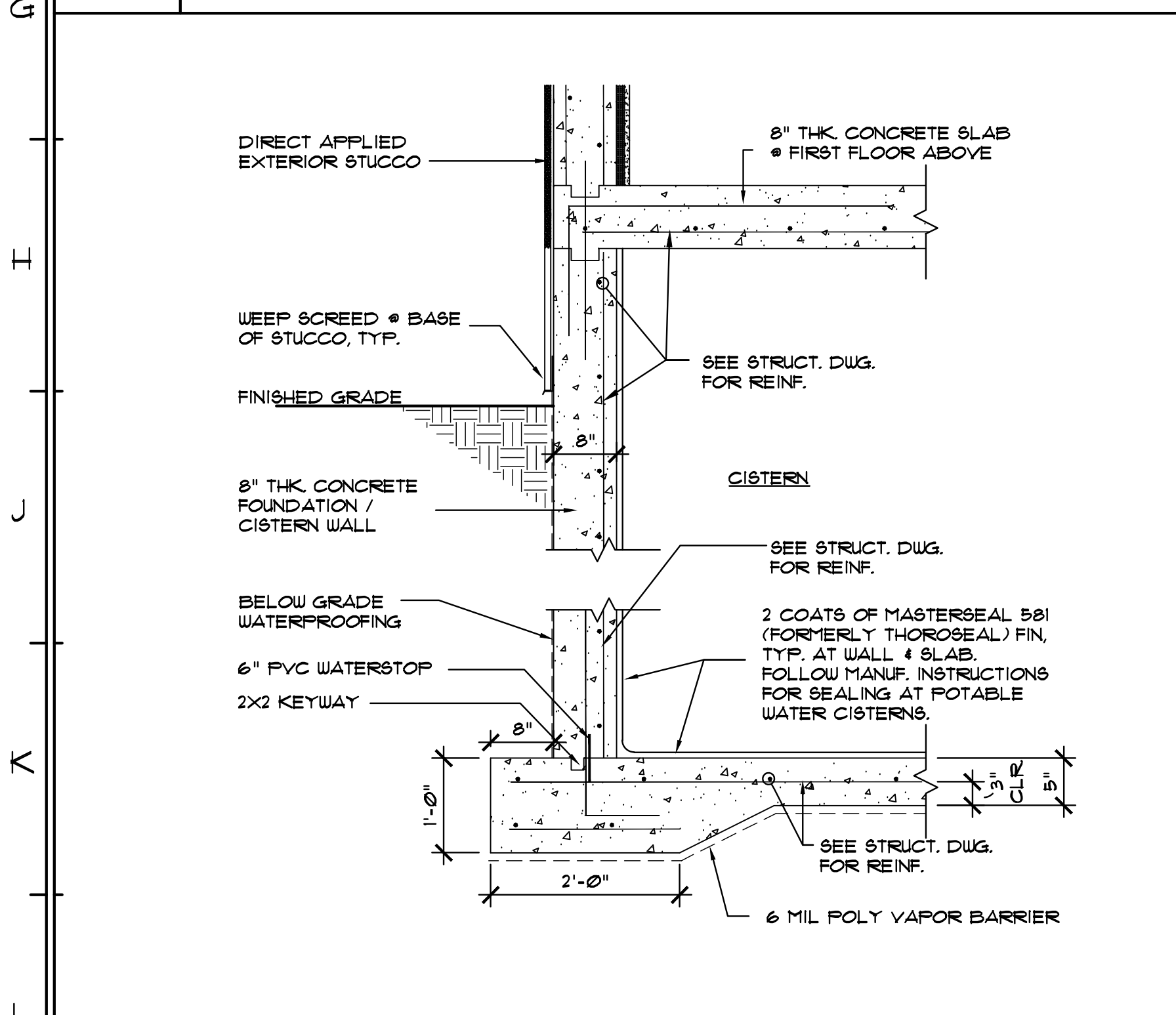
L1 CISTERN WALL DETAIL
