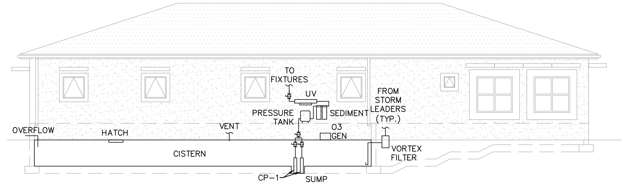
CISTERN DETAIL
