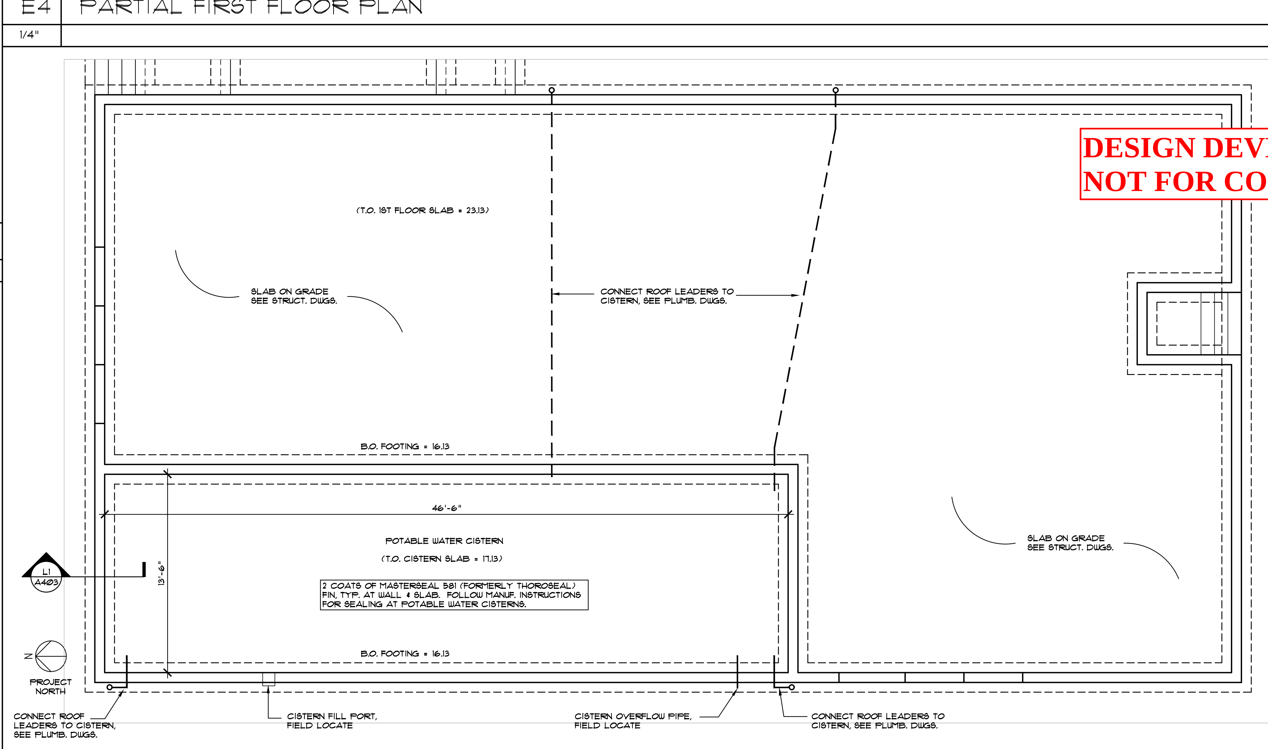
L4 FLOOR PLAN
