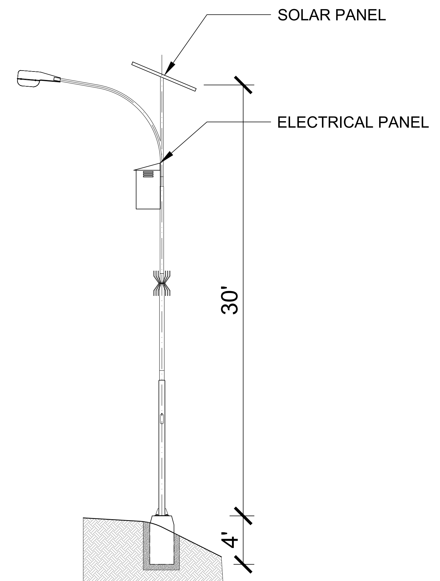
SITE LIGHTING DETAIL 2 SCALE: NTS
