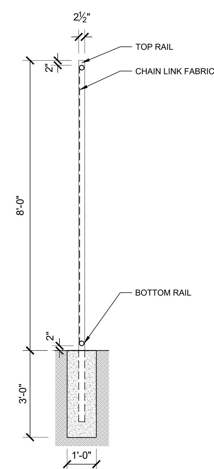
PERIMETER CHAINLINK FENCE 3 SCALE: 1/2" = 1'-0"
